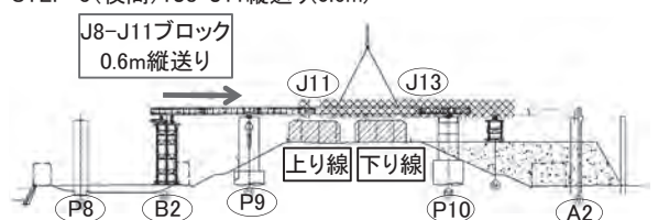
STEP-3(夜間): J8-J11縦送り(0.6m)
